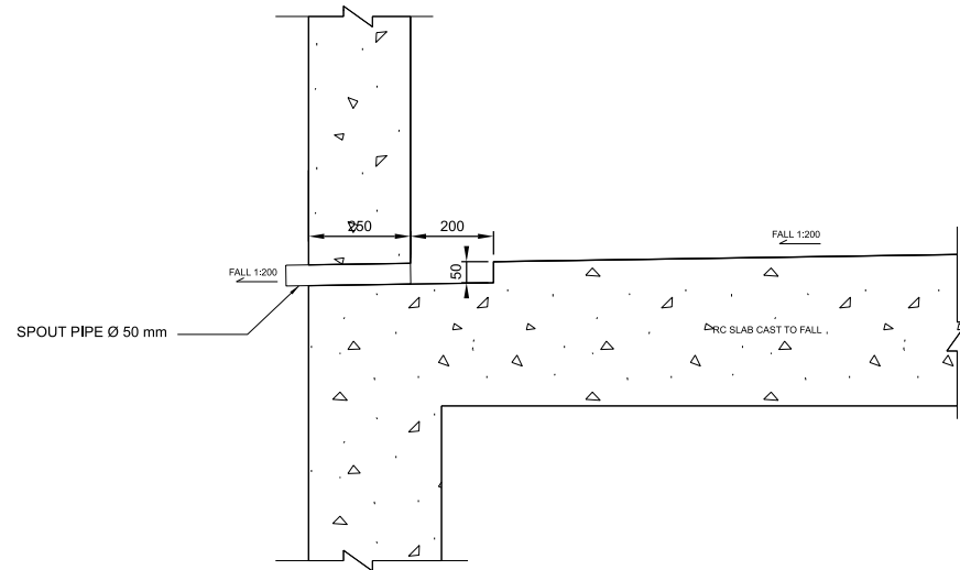
TYP. WATERPROOFING DETAIL - SECTION A1-A1 SPOUT PIPE DISCHARGE 1:10
