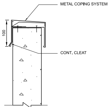
TYP. WATERPROOFING DETAIL PARAPET WALL 1:5
