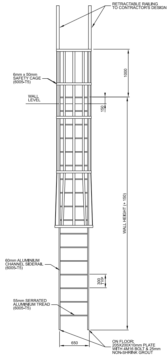
CAT LADDER WITH RETRACTABLE HANDLE 1:25
