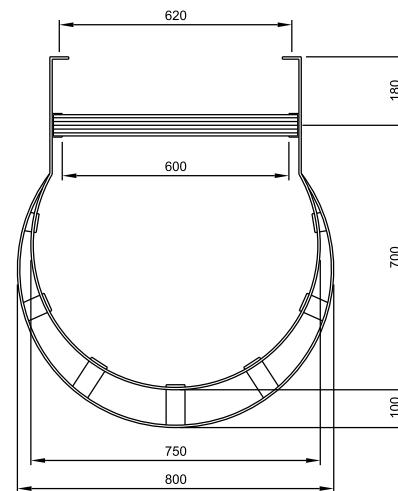
CAT LADDER PLAN (PARAPET PLATFORM & RETURN LADDER ARE OMITTED FOR CLARITY)
