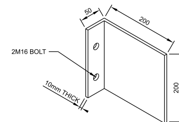
CAT LADDER DETAIL BRACKET DETAIL TO STRUCTURE ON TOP FACTORY FINISH ALUMINIUM-MILL FINISH
