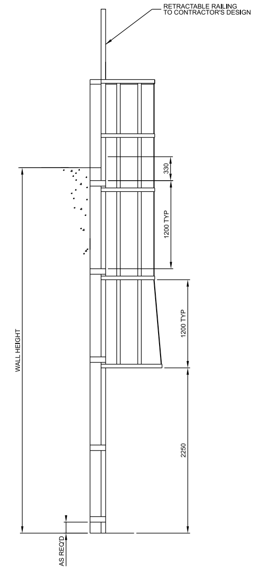
CAT LADDER WITH RETRACTABLE HANDLE 1:25
